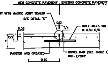
DETAIL OF CONSTRUCTION JOINT DETAIL OF JOINT BETWEEN NEW AND EXISTING CONCRETE PAVEMENT NOT TO SCALE
