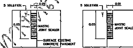
DETAIL OF SAWS FOR LONGITUDINAL JOINT NOT TO SCALE
