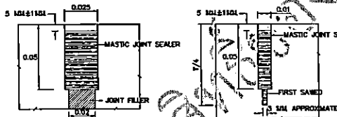
DETAIL "A" (EXPANSION JOINT) DETAIL "B" (CONTRACTION JOINT)
