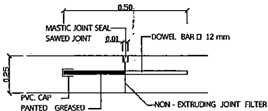
EXPANSION JOINT
