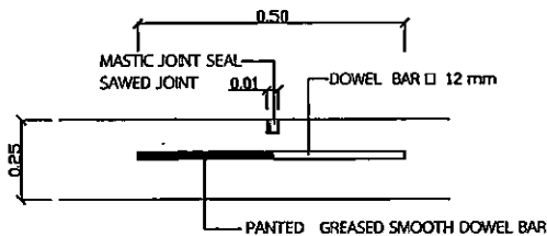
CONTRACTION JOINT
