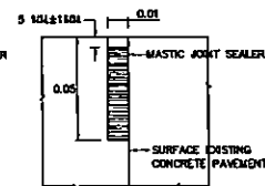
DETAIL "C" (CONSTRUCTION JOINT)
